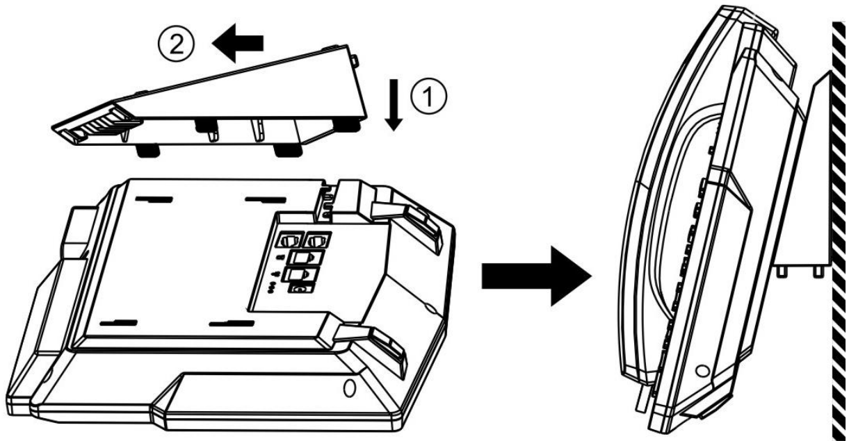
Figure 3 - Wall-mount Installation
